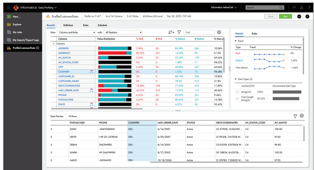
Figure 3: Informatica Data Quality provides data profiling to enable Data Stewards to analyze data patterns and values. This helps identify quality issues and build business rules for further analysis and remediation.
