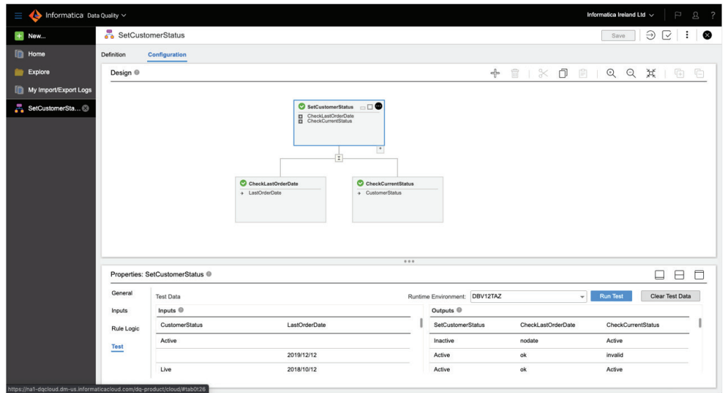
Figure 1: The Informatica Analyst Tool has a Business Rule Specification feature, which allows data stewards and other data experts to create custom data quality rules to implement business requirements.
